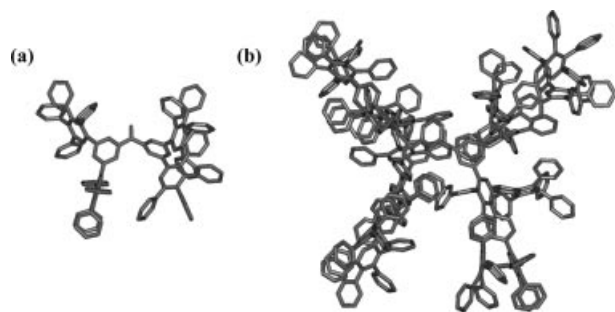
Figure 1. Molecular model of (a) the first-generation dendrimer 8 and (b) the second-generation dendrimer 12 . For reasons of clarity, the hydrogen atoms have been omitted. Radii were measured as largest carbon–carbon distances between the carbonyl carbon and peripheral benzene rings.
