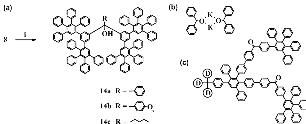
Scheme 3. (a) Chemical functionalizations of the first-generation dendrimer 8 with aryl- and alkylolithium and Grignard reagents. (b) Potassium-bridged biradical of benzophenone. (c) Schematic drawing of a polyphenylene dendrimer functionalized with eight benzophenones in the scaffold. [6] One arm is drawn out fully. The three other arms are identical with the one shown but are abbreviated as a circled-D for ease of visualization. (i) 14a : 60 equiv. phenyllithium, THF, 70 °C, 70%. 14b : 25 equiv. (4-methoxyphenyl)magnesium bromide, THF, 70 °C, 66%. 14c : 100 equiv. n -butyllithium, THF, 70 °C, 70%.
