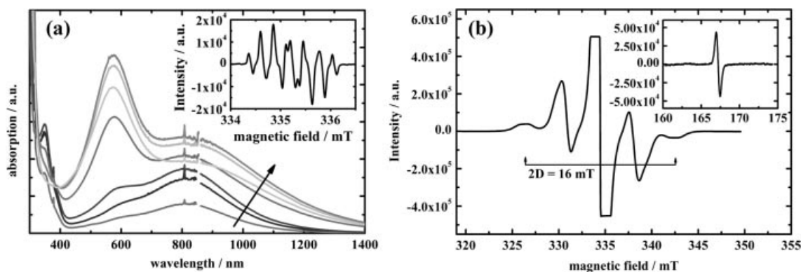
Figure 2. (a) UV/Vis absorption spectra of dendrimer 8 in THF in the order of further reduction. (K, THF, room temp.) Inset: EPR spectrum of dendrimer 8 at the maximum amount of radical monoanion. (b) EPR spectra of the radical anion of 8 in THF at ca. 120 K, zero-field splittings and half-field transition (inset).
