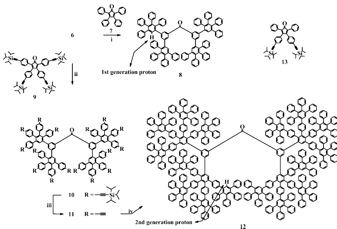
Scheme 2. Synthesis of the first- and second-generation dendrimers 8 and 12 , (i) 6 equiv. 7 , o -xylene, 150 °C, 77%. (ii) 6 equiv. 9 , o -xylene, 160 °C, 76%; (iii) TBAF, THF, 78%; (iv) 48 equiv. 7 , o -xylene, 170 °C, 85%.
