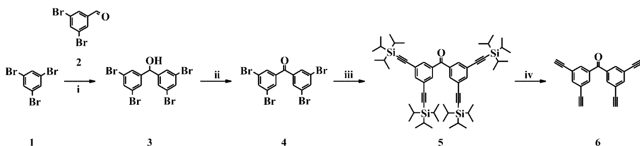
Scheme 1. Synthesis of the benzophenone core 3,3',5,5'-(tetraethynyl)benzophenone ( 6 ). (i) n -butyllithium, -78 °C, 80%; (ii) oxalyl chloride, DMSO, triethylamine, CH_2Cl_2 , -78 °C, 85%; (iii) 6 equiv. (triisopropylsilyl)ethyne, [Pd(PPh_3)_2]Cl_2 , PPh_3 , CuI, toluene/triethylamine, 80 °C, 60%; (iv) TBAF, THF, 67%.
